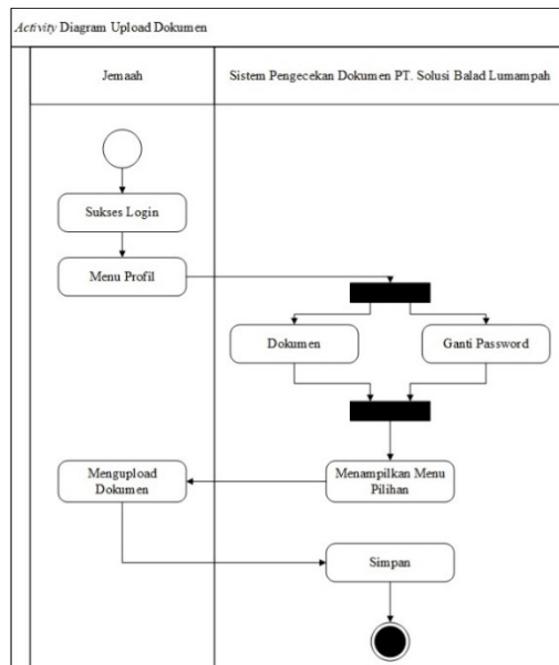
Gambar 10 Activity diagram upload dokumen
