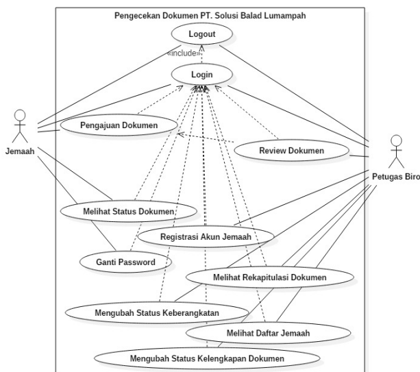
Gambar 8 Use Case diagram sistem
